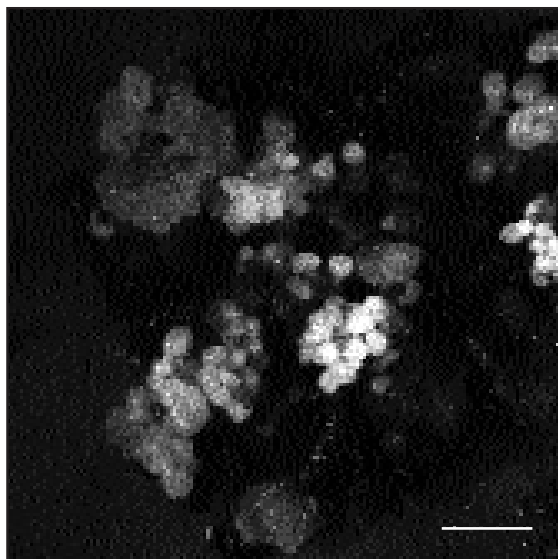
Figure 2. American chestnut embryonic material approximately 2 weeks following removal from liquid nitrogen, showing some regrowth. Bar = 2 mm.
