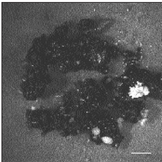
Figure 1. American chestnut embryonic material approximately 1 week following removal from liquid nitrogen. Bar = 2 mm.
