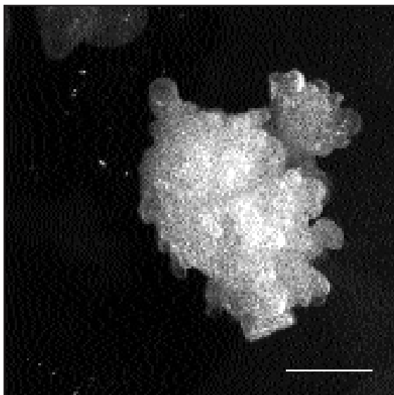
Figure 3. American chestnut embryonic material approximately 3 weeks following removal from liquid nitrogen, showing some regrowth. Bar = 1 mm.
