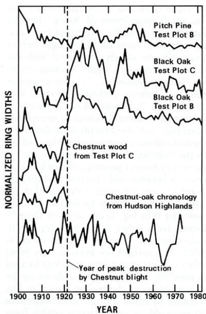
Tree ring chronology of chestnut blight.
