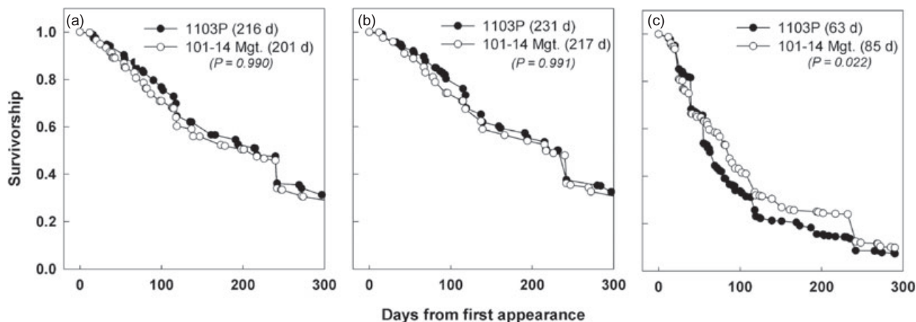
Figure 5. Root survivorship in a vineyard in Oakville, California for (a) total, (b) uninfested and (c) phyloxera-infested roots of a rootstock with fast (1103P) and slow (101-14 Mgt) growth rates. Median lifespans are indicated in parentheses. Data are for all roots observed through minirhizotron windows located in both irrigated and non-irrigated soils in 2002 and 2003. The rootstock of slower growth rate, which produced fewer roots, had significantly higher root survivorship ( P = 0.022 ). Differences in survivorship between uninfested (b) and infested (c) roots were significant for both root systems ( P < 0.001 ).
