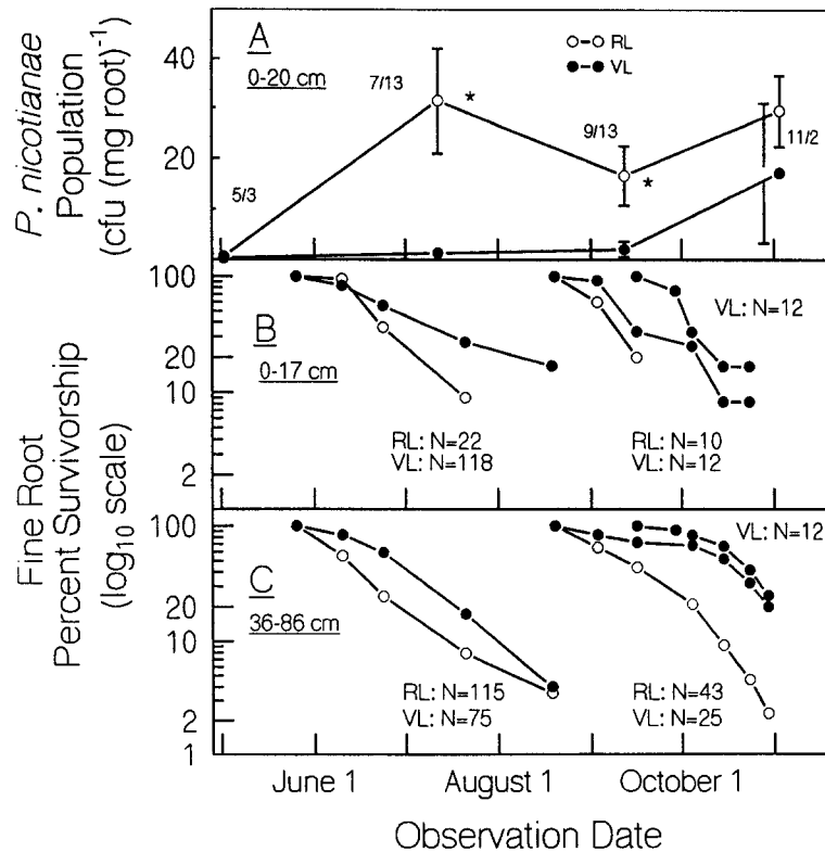
Fig. 1. A) Populations of Phytophthora nicotianae (colony forming units (cfu) per mg root) in soil cores from 0–20 cm depth. Samples taken from May 3, 1993 to Nov. 2, 1993; N = 8 . Starred values at each date are significantly different ( p < 0.05 ); ANOVA done on log-transformed data. Error bars are \pm standard error of the mean; error bars not shown fall within the symbol. RL = Rough lemon; VL = Volkamer lemon. B) Percent of the initial population surviving at each observation date (survivorship) for cohorts of rough lemon fine roots (open symbols) and Volkamer lemon fine roots (closed symbols) from 0 to 17 cm depth from the soil surface. The earliest cohort of roots appeared between May 5 and June 10, 1993; root age estimates are \pm 33 days. The August cohort of roots appeared between August 4 and September 1, 1993; root age estimates are \pm 17–28 days. The September cohort of roots appeared between September 1 and September 30; root age estimates are \pm 17–20 days. Note the logarithmic scale of the ordinate. C) Survivorship curves for cohorts of rough lemon fine roots (open symbols) and Volkamer lemon roots (closed symbols) from 36 to 86 cm depth from the soil surface. Cohort appearance dates as above.
