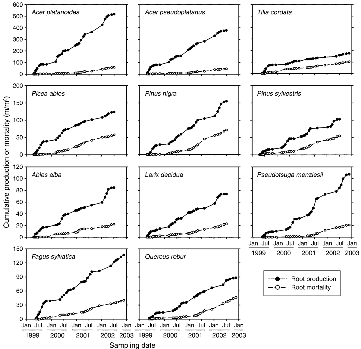
FIG. 1. Cumulative production and cumulative mortality of fine roots (first- and second-order roots only) against minirhizotron tubes from May 1999 to November 2002, averaged across plots (two, three, or six plots per species). The mean difference between production and mortality can be found in Table 3. Note the difference in the y-axis scales. Our field site was a common garden planting in the Siemianice Experimental Forest in central Poland.
