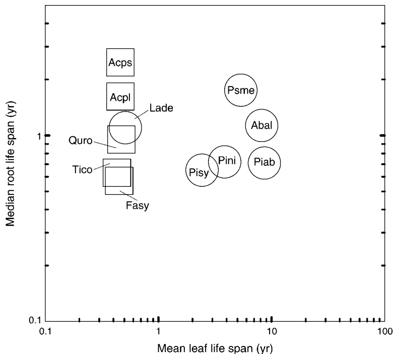
FIG. 2. Relationship of fine-root life span to leaf life span (note log scales). Hardwoods are denoted by squares, and conifers by circles. Species abbreviations are the first two letters of the genus and species. Picea abies is plotted as the mean of the two sites for leaf life span.
