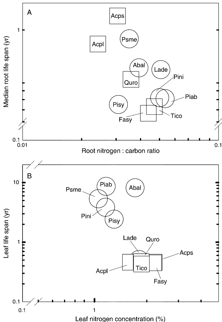
FIG. 3. The relationships between (A) longevity in roots and nitrogen : carbon ratio and (B) longevity in leaves and nitrogen concentration. Traits are on a log-log scale. Hardwoods are denoted by squares, and conifers by circles. Species abbreviations are the first two letters of the genus and species.
