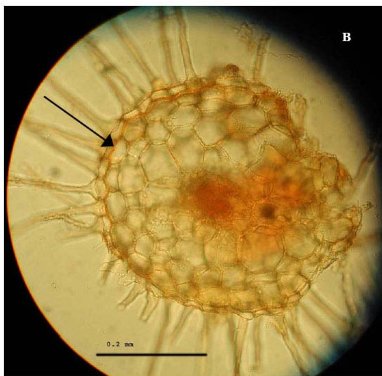
FIG. D1. (A) Cross-section of a first-order Acer pseudoplatanus root stained with 0.05% phloroglucinol. The xylem and the thickened walls of the exodermis are stained red, and the latter is marked with an arrow. (B) Cross-section of a white first-order Picea abies root stained with 0.05% phloroglucinol. The exodermis is stained red and marked with an arrow.
