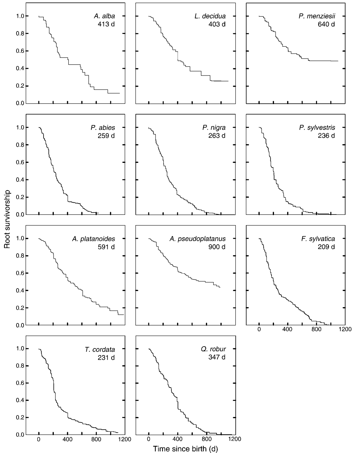
FIG. 4. Root survivorship curves from minirhizotron data for each species. Root birth and death are estimated as halfway between successive sampling dates from when a root was not present to the date it first appeared. Cox proportional hazards models were run with depth in soil, diameter, and pigmentation held constant. Median root survivorship is noted for each species.
