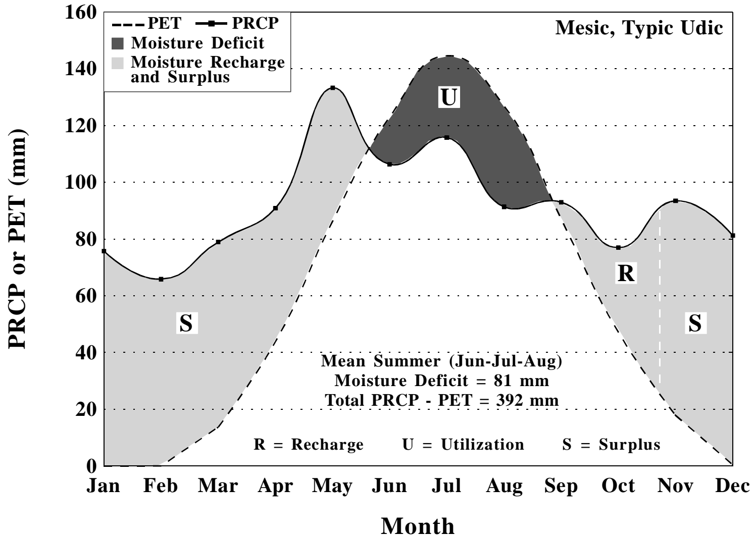
Moisture balance for Lebanon 2 W, Pennsylvania, based upon a period of 1961-1990. PET calculated by Newhall Simulation Model (Van Wambeke et al., 1992).
