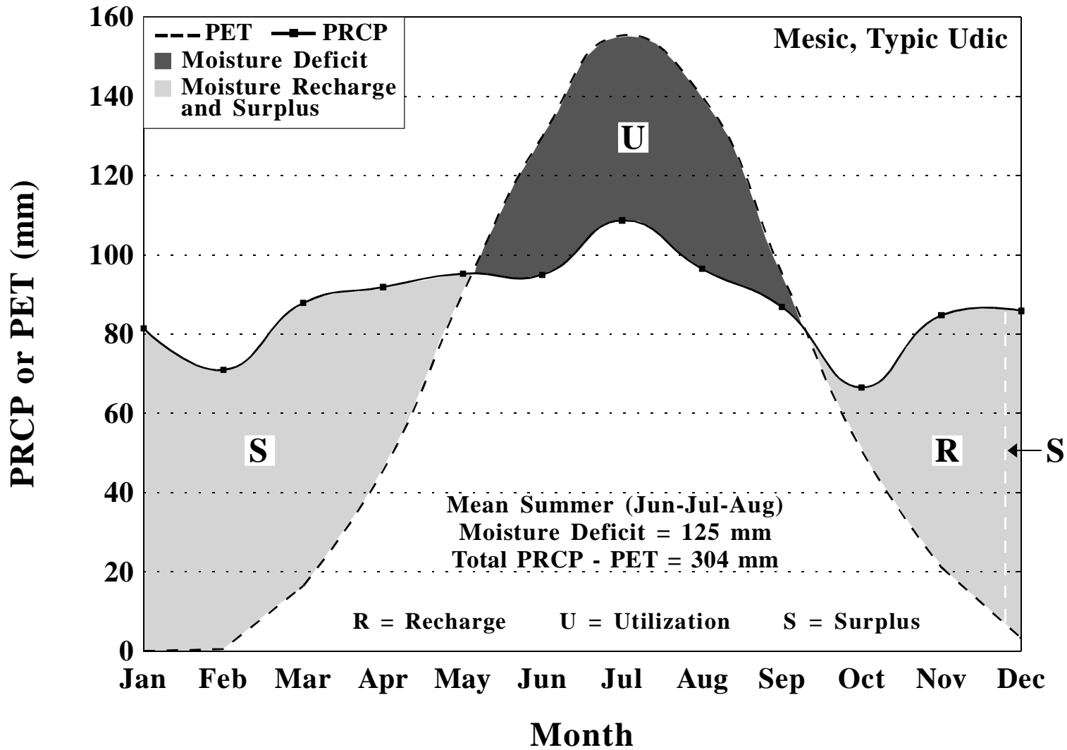
Moisture balance for Philadelphia WSCMO Airport, Pennsylvania, based upon a period of 1961-1990. PET calculated by Newhall Simulation Model (Van Wambeke et al., 1992).
