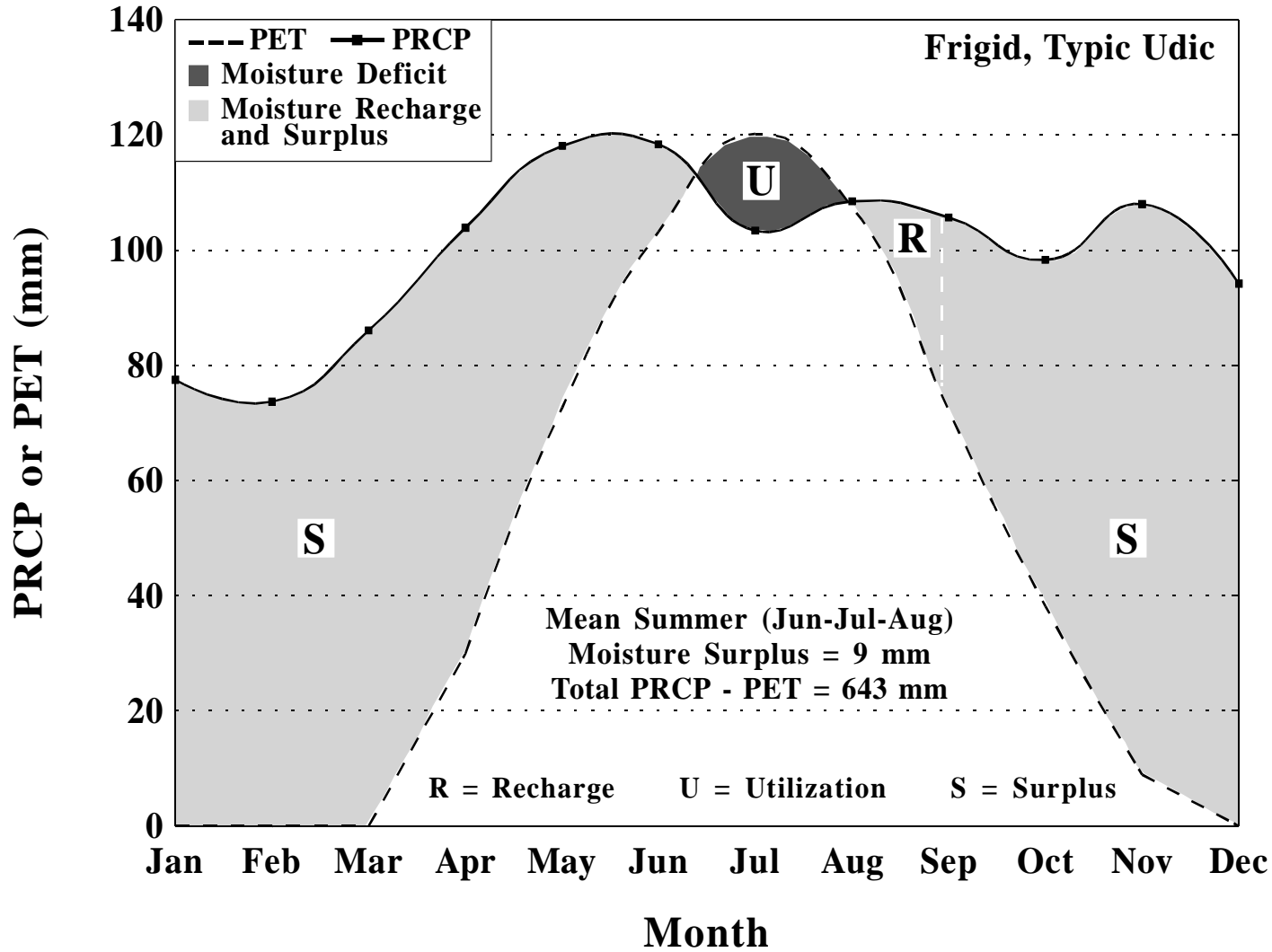
Moisture balance for Pleasant Mount 1 W, Pennsylvania, based upon a period of 1961-1990. PET calculated by Newhall Simulation Model (Van Wambeke et al., 1992).
