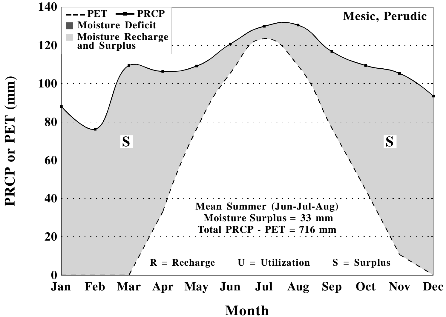
Moisture balance for Mount Pocono 2 N, Pennsylvania, based upon a period of 1927-1960. PET calculated by Newhall Simulation Model (Van Wambeke et al., 1992).
