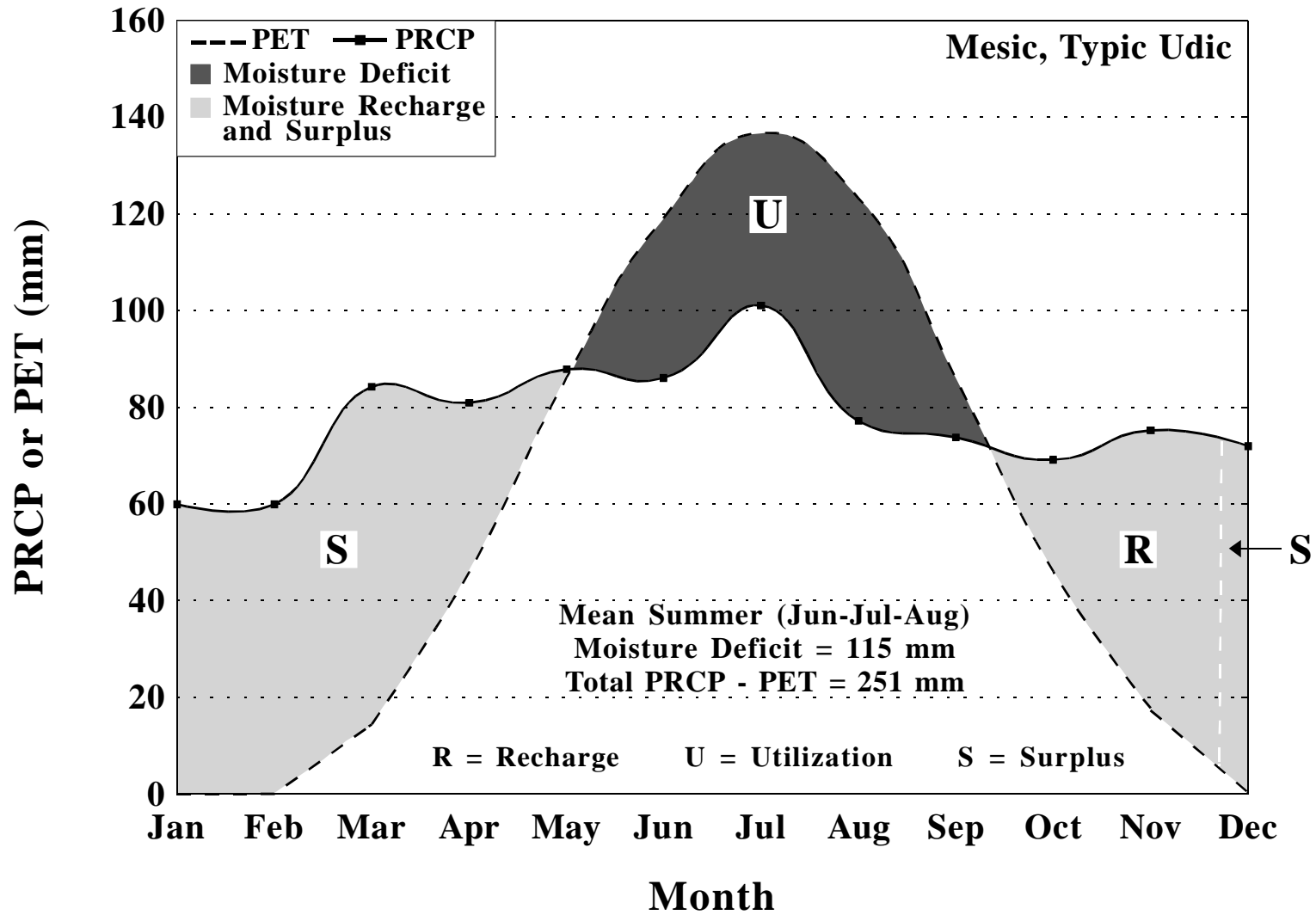
Moisture balance for Kegg, Pennsylvania, based upon a period of 1961-1990. PET calculated by Newhall Simulation Model (Van Wambeke et al., 1992).
