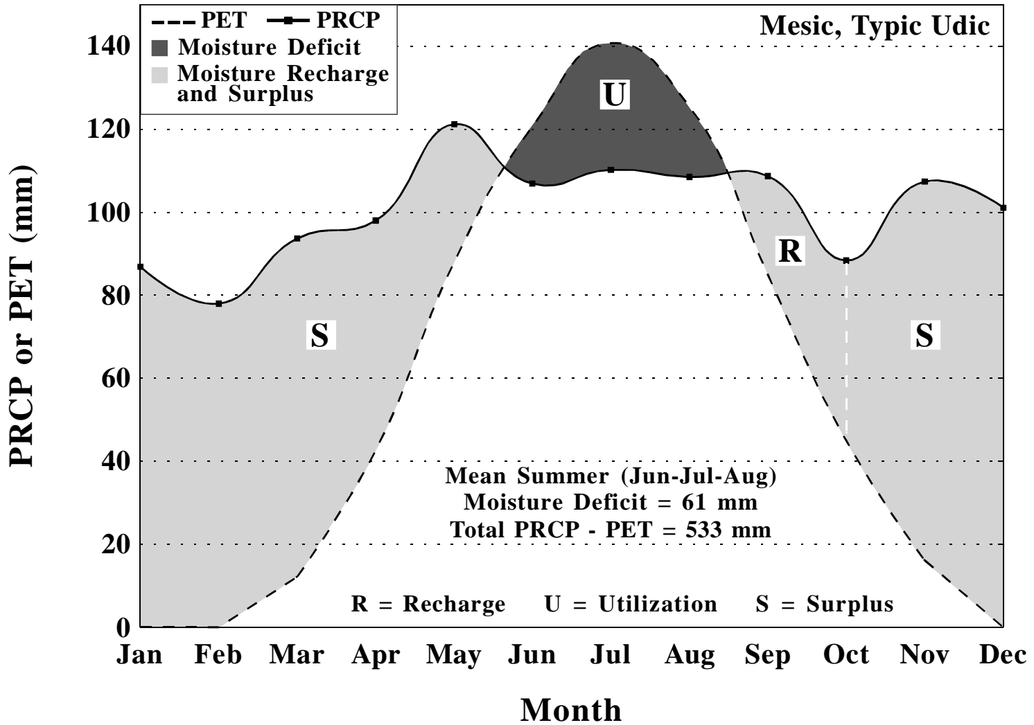
Moisture balance for Stroudsburg, Pennsylvania, based upon a period of 1961-1990. PET calculated by Newhall Simulation Model (Van Wambeke et al., 1992).
