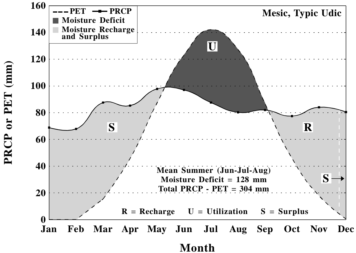
Moisture balance for Chambersburg 1 ESE, Pennsylvania, based upon a period of 1961-1990. PET calculated by Newhall Simulation Model (Van Wambeke et al., 1992).
