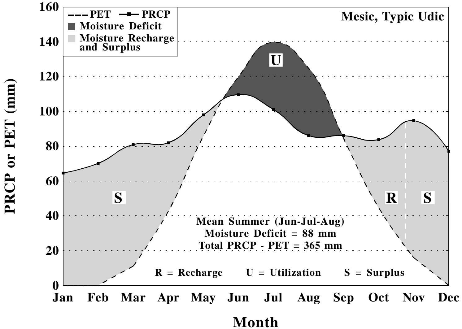
Moisture balance for Williamsport WSO Airport, Pennsylvania, based upon a period of 1961-1990. PET calculated by Newhall Simulation Model (Van Wambeke et al., 1992).
