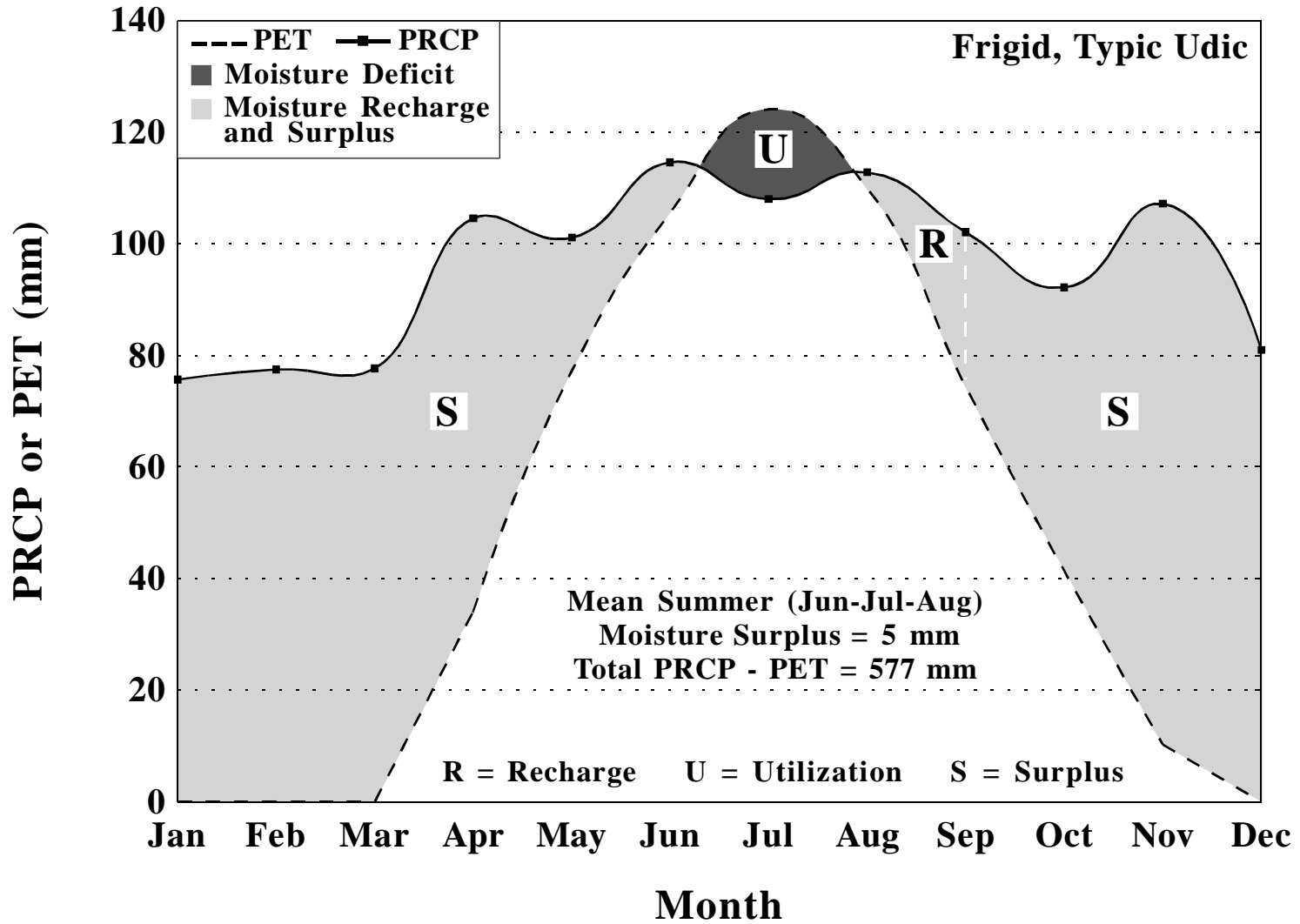
Moisture balance for Eagles Mere, Pennsylvania, based upon a period of 1949-1987. PET calculated by Newhall Simulation Model (Van Wambeke et al., 1992).
