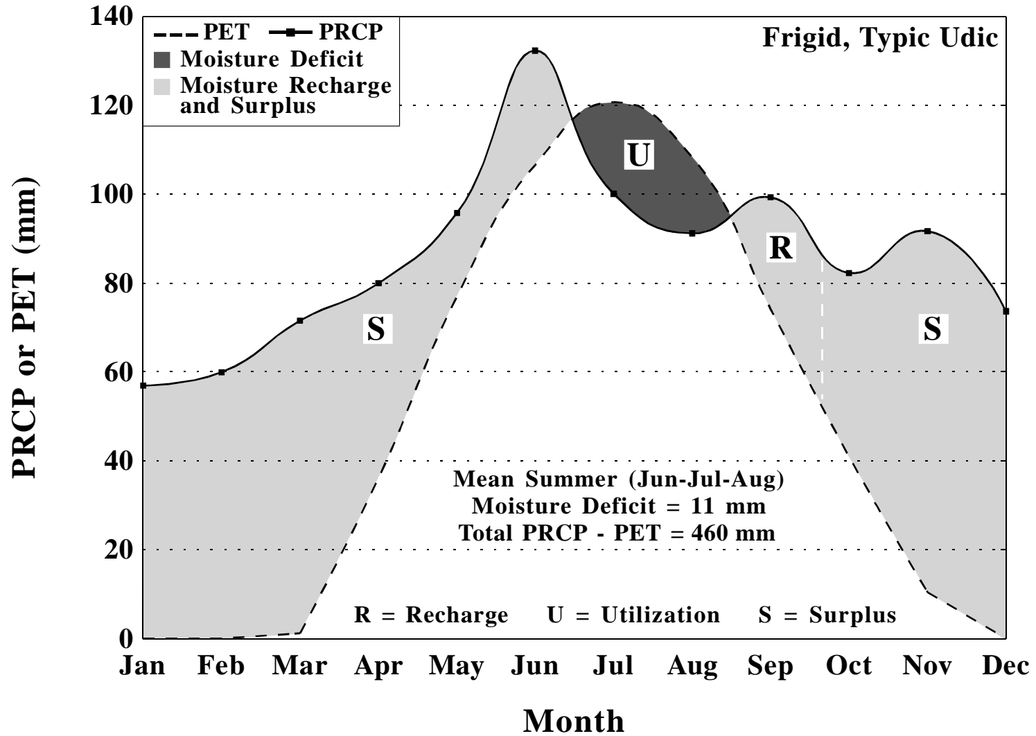
Moisture balance for Coudersport 4 NW, Pennsylvania, based upon a period of 1961-1990. PET calculated by Newhall Simulation Model (Van Wambeke et al., 1992).
