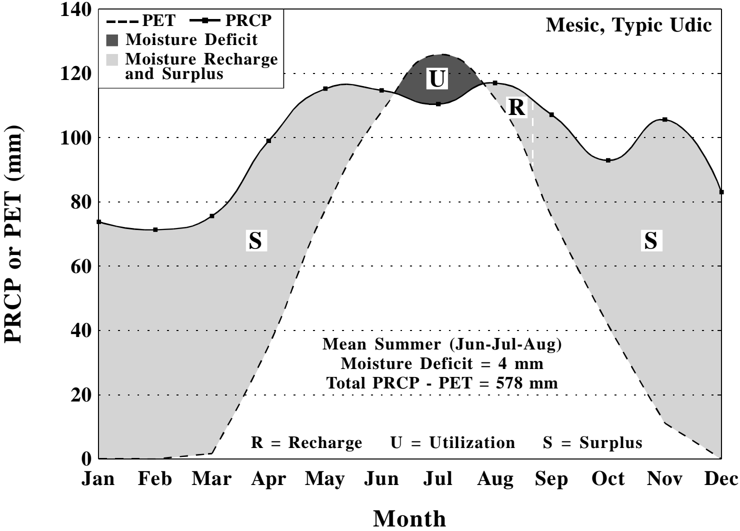
Moisture balance for Freeland, Pennsylvania, based upon a period of 1961-1990. PET calculated by Newhall Simulation Model (Van Wambeke et al., 1992).
