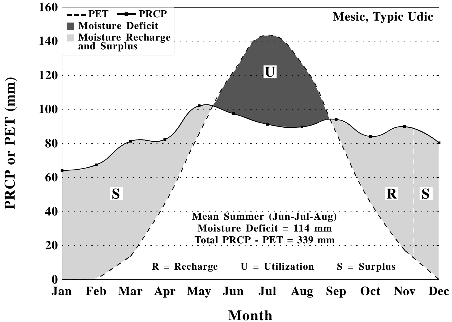
Moisture balance for Newport, Pennsylvania, based upon a period of 1961-1990. PET calculated by Newhall Simulation Model (Van Wambeke et al., 1992).
