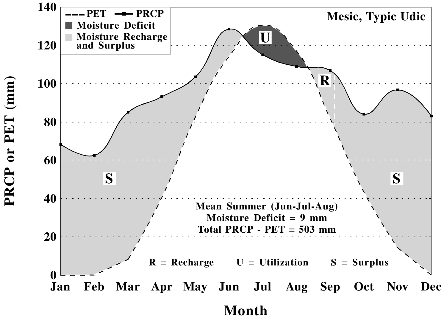
Moisture balance for Clarion 3 SW, Pennsylvania, based upon a period of 1961-1990. PET calculated by Newhall Simulation Model (Van Wambeke et al., 1992).
