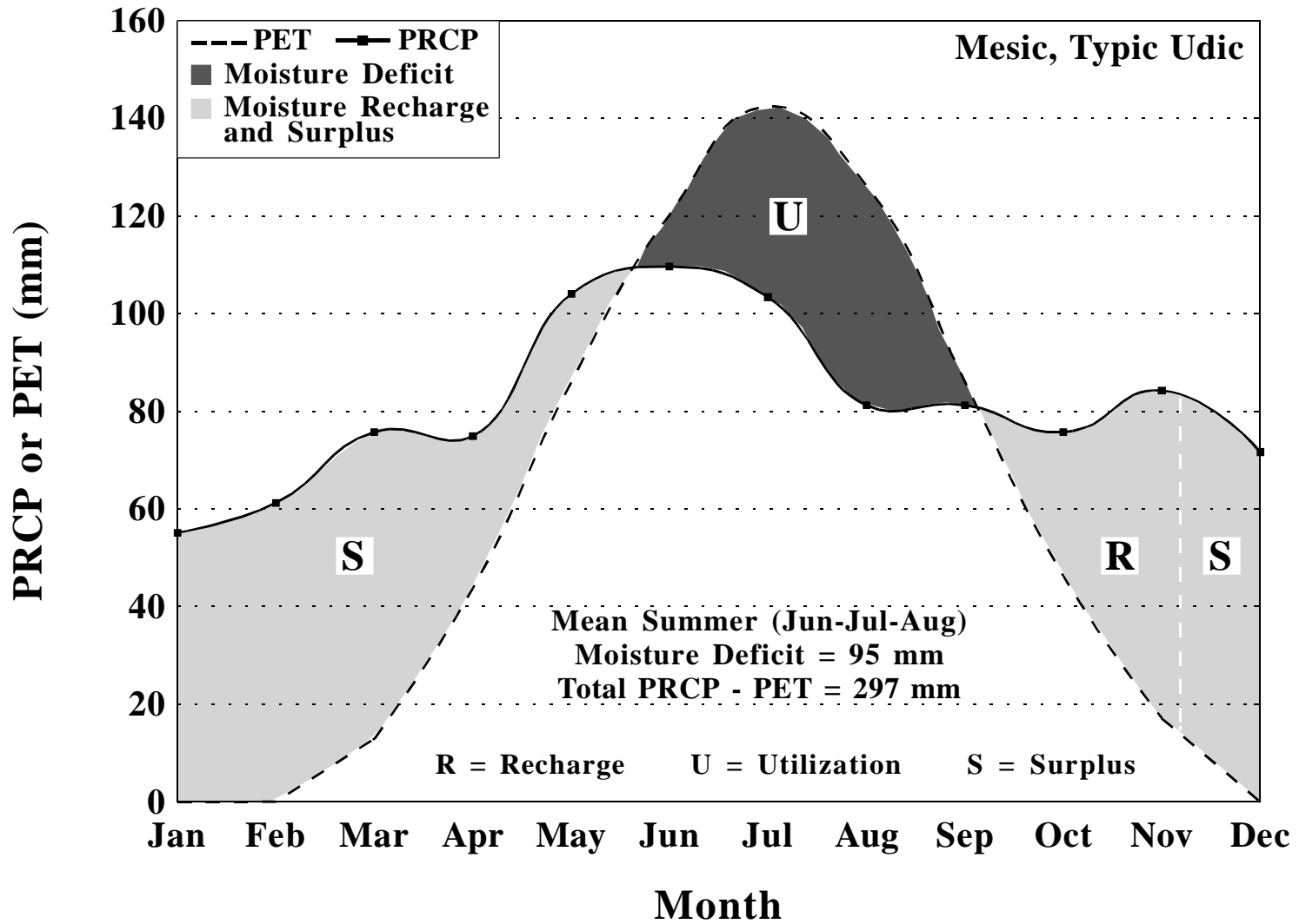
Moisture balance for Lewistown, Pennsylvania, based upon a period of 1961-1990. PET calculated by Newhall Simulation Model (Van Wambeke et al., 1992).
