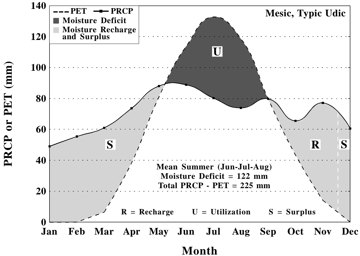
Moisture balance for Towanda 1 ESE, Pennsylvania, based upon a period of 1961-1990. PET calculated by Newhall Simulation Model (Van Wambeke et al., 1992).
