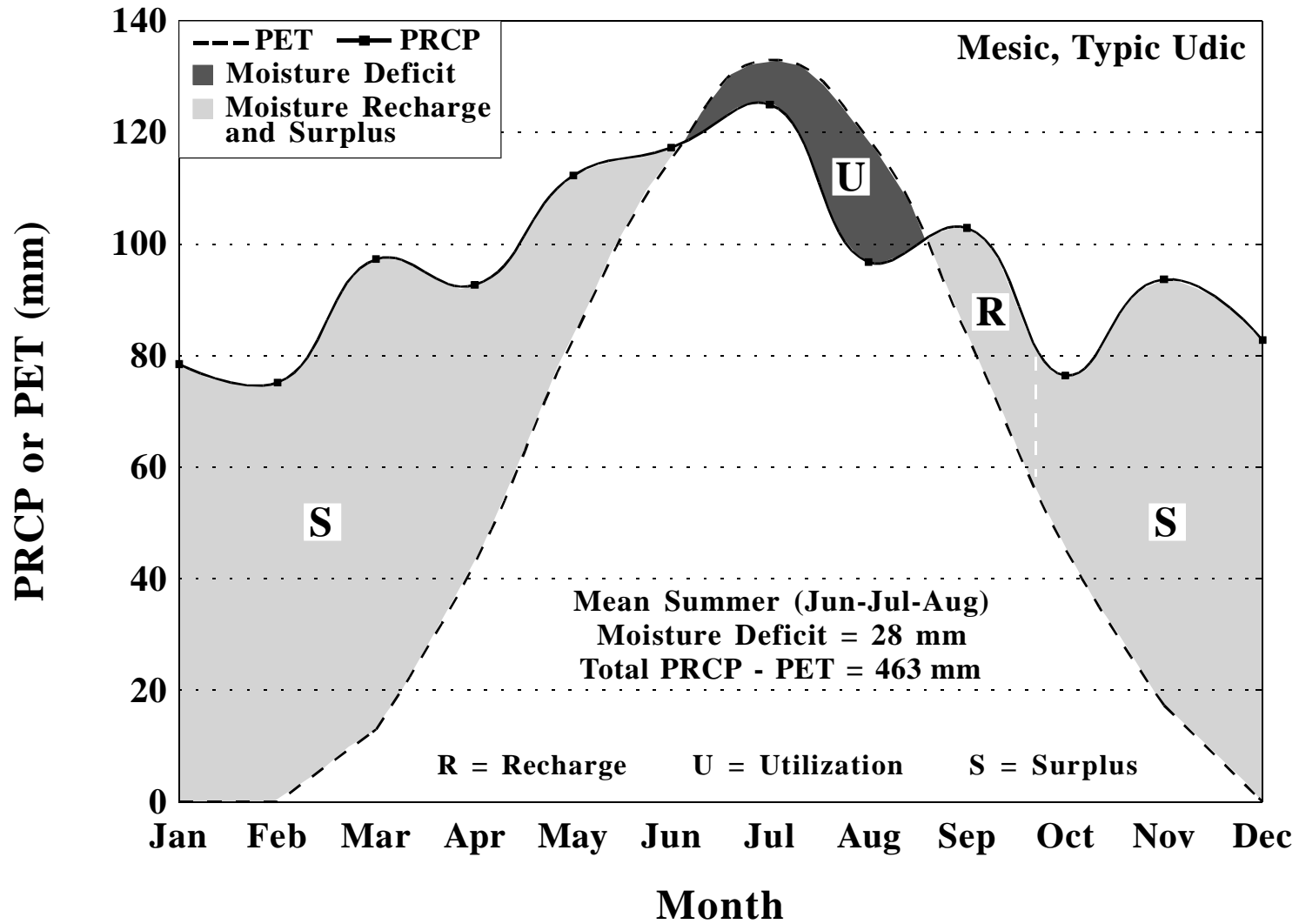
Moisture balance for Indiana 3 SE, Pennsylvania, based upon a period of 1961-1990. PET calculated by Newhall Simulation Model (Van Wambeke et al., 1992).
