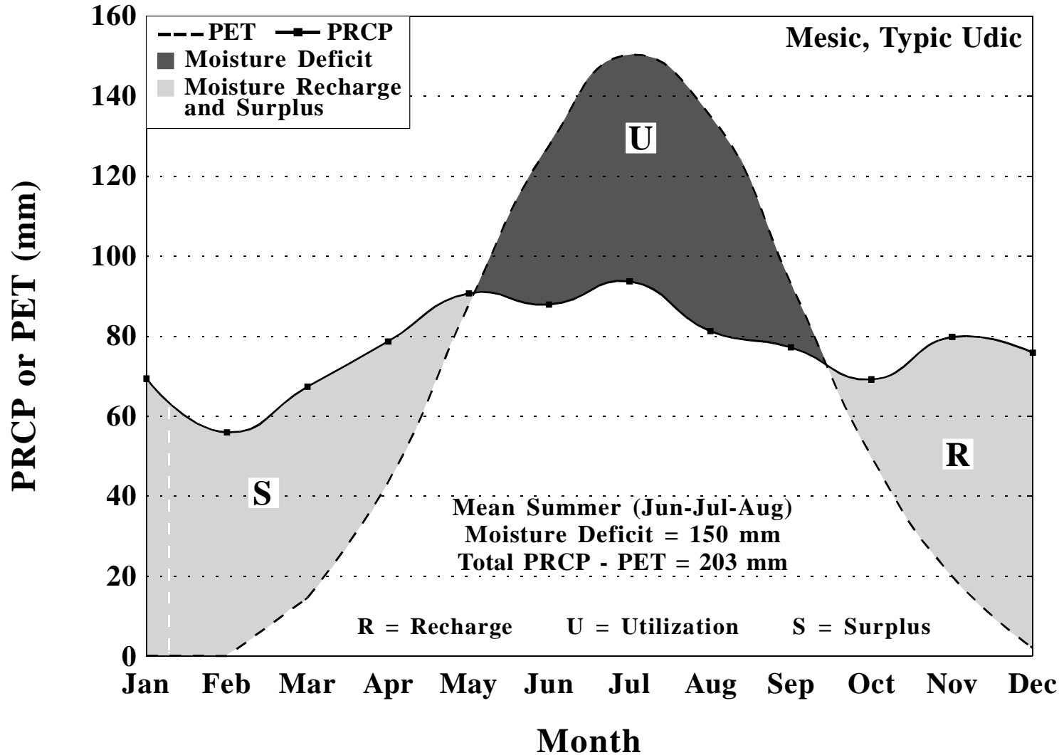
Moisture balance for Holtwood, Pennsylvania, based upon a period of 1961-1990. PET calculated by Newhall Simulation Model (Van Wambeke et al., 1992).
