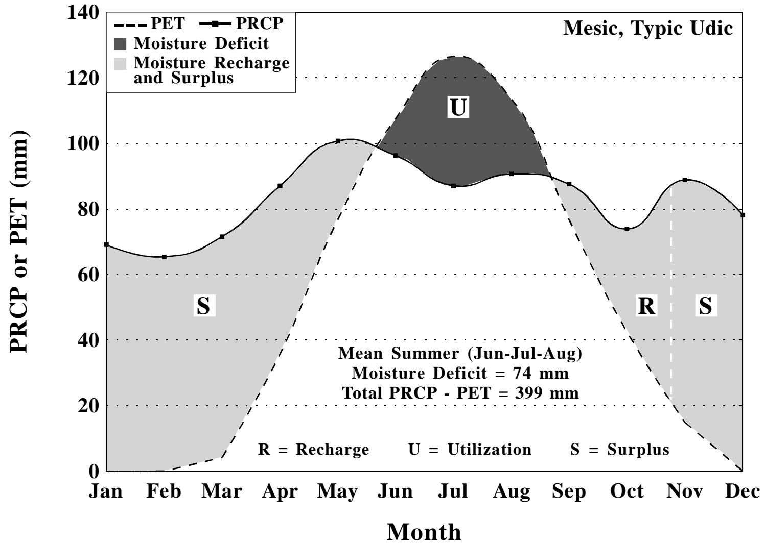
Moisture balance for Hawley 1 E, Pennsylvania, based upon a period of 1961-1990. PET calculated by Newhall Simulation Model (Van Wambeke et al., 1992).
