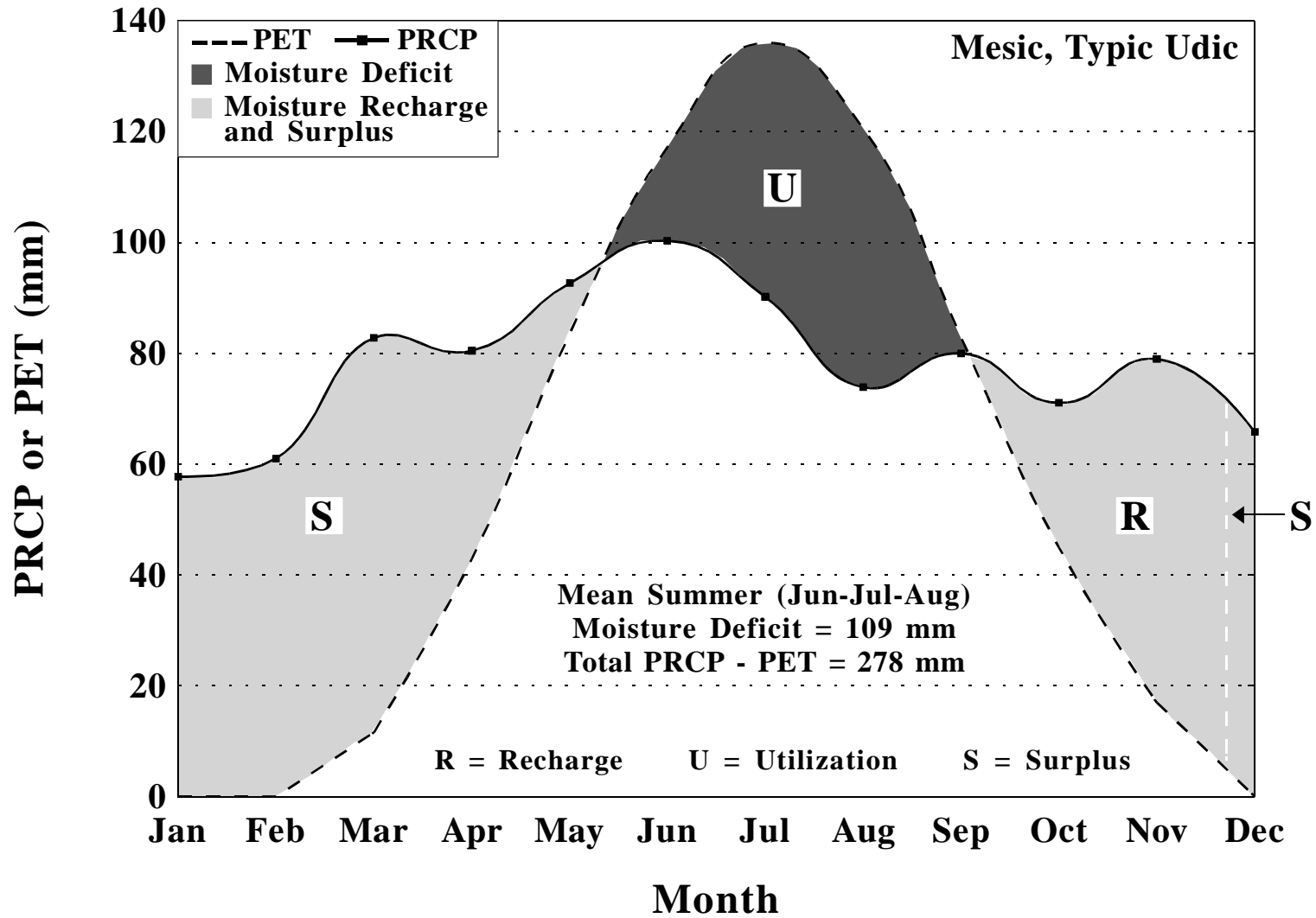
Moisture balance for Altoona FAA Airport, Pennsylvania, based upon a period of 1961-1990. PET calculated by Newhall Simulation Model (Van Wambeke et al., 1992).
