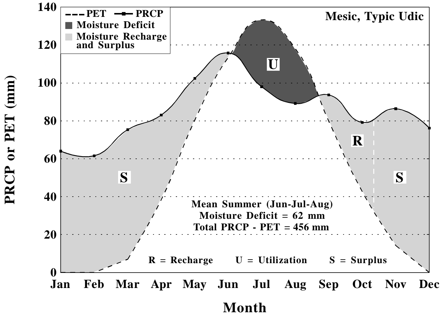
Moisture balance for Millville 2 SW, Pennsylvania, based upon a period of 1961-1990. PET calculated by Newhall Simulation Model (Van Wambeke et al., 1992).
