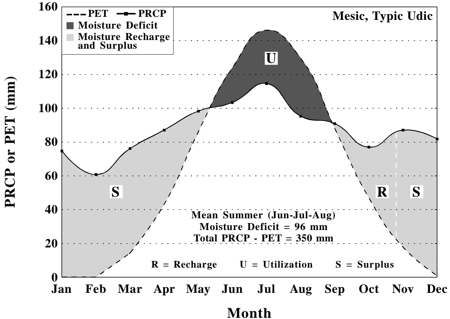
Moisture balance for Lancaster 2 NE, Pennsylvania, based upon a period of 1961-1990. PET calculated by Newhall Simulation Model (Van Wambeke et al., 1992).
