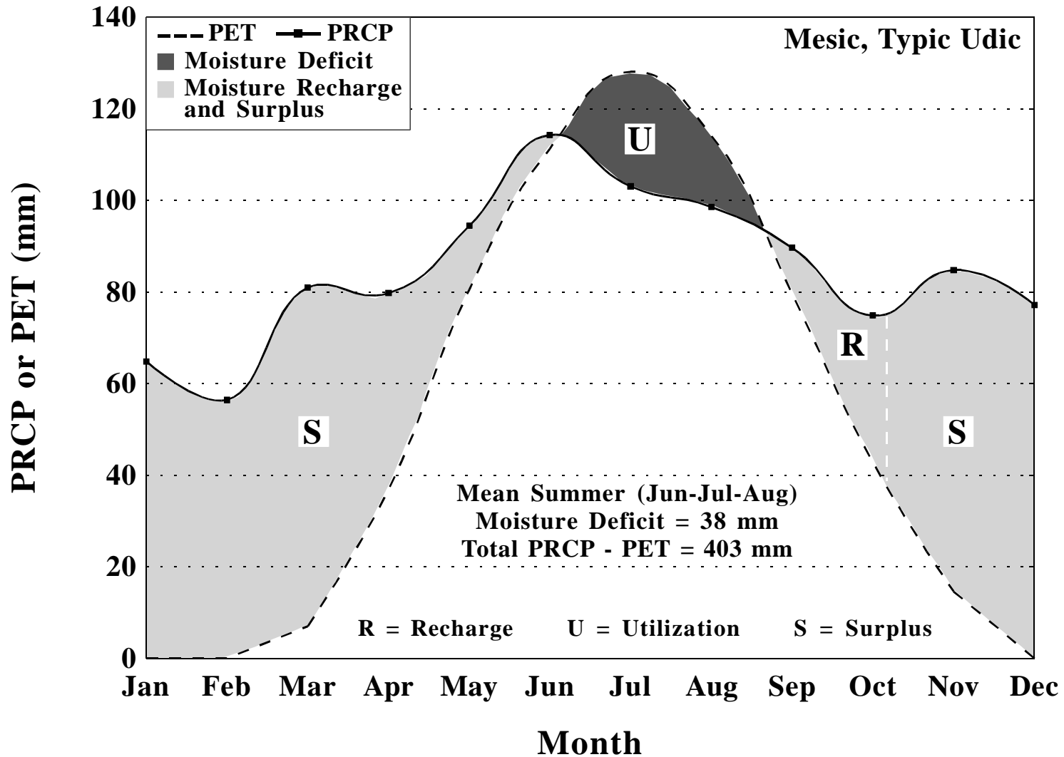
Moisture balance for Slippery Rock 1 SSW, Pennsylvania, based upon a period of 1961-1990. PET calculated by Newhall Simulation Model (Van Wambeke et al., 1992).
