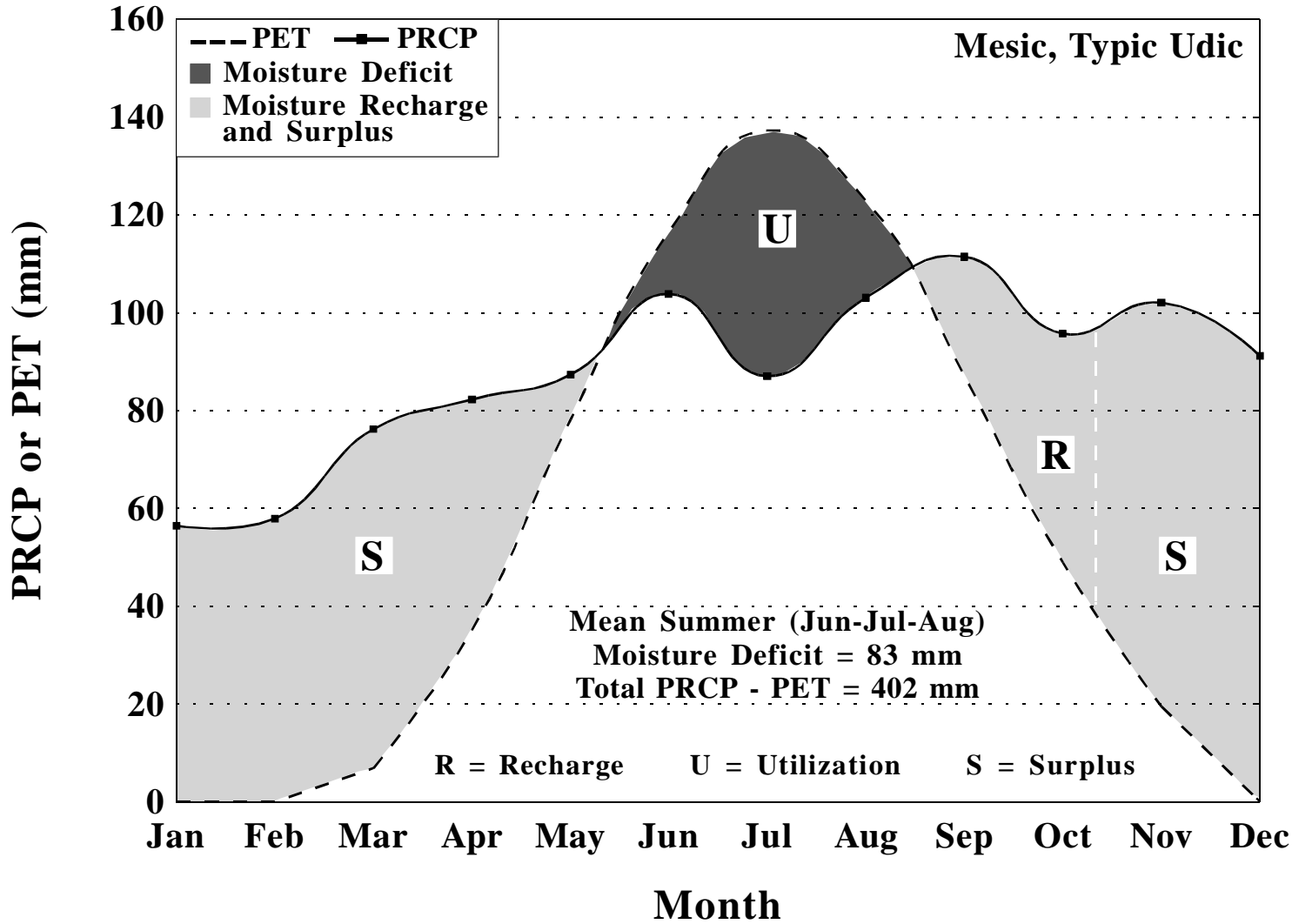
Moisture balance for Erie WSO Airport, Pennsylvania, based upon a period of 1961-1990. PET calculated by Newhall Simulation Model (Van Wambeke et al., 1992).
