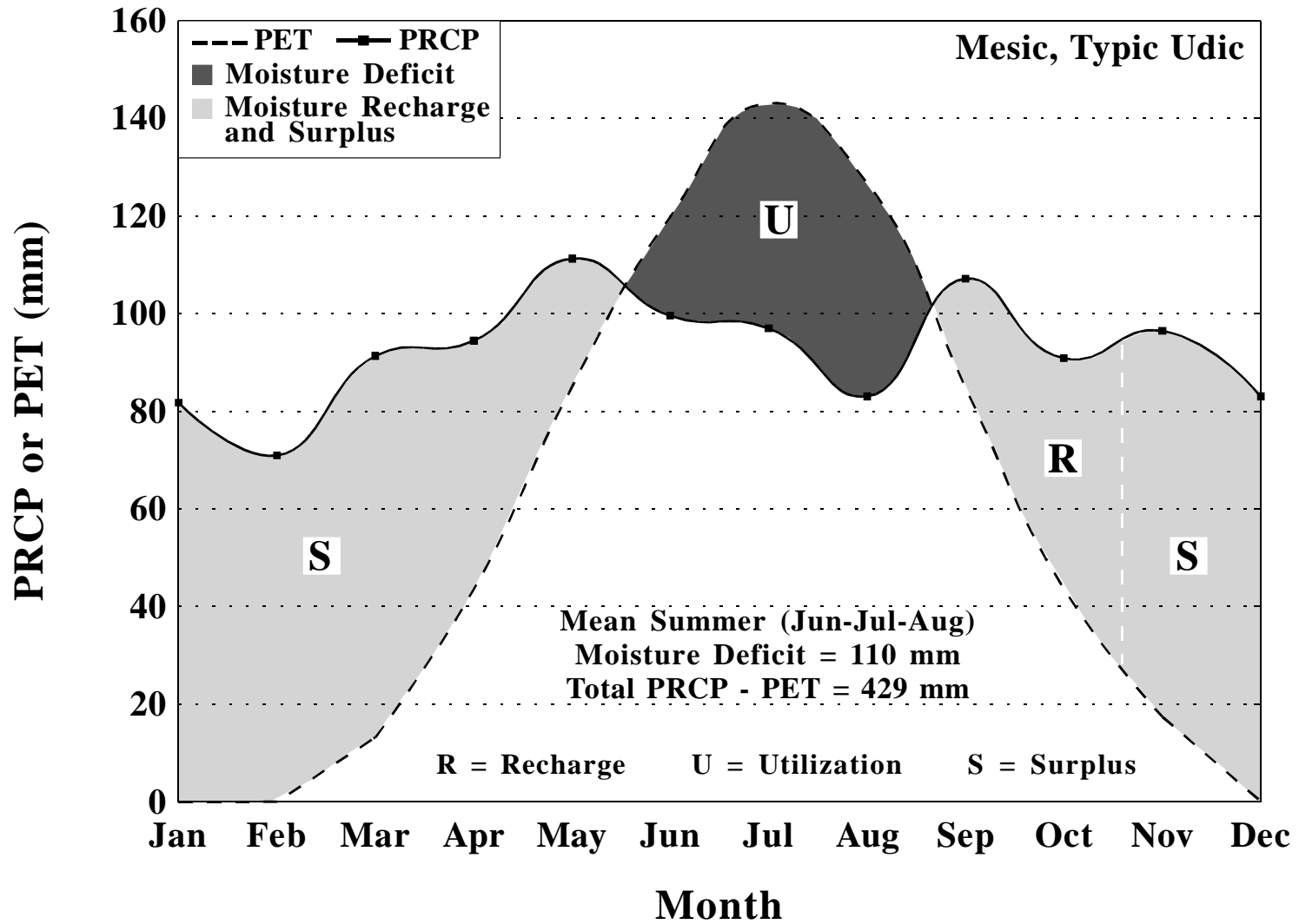
Moisture balance for Biglerville, Pennsylvania, based upon a period of 1972-1995. PET calculated by Newhall Simulation Model (Van Wambeke et al., 1992).
