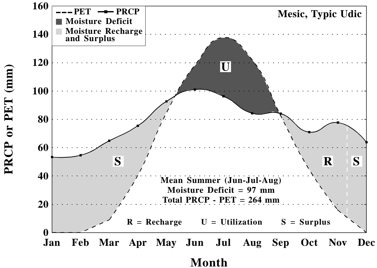
Moisture balance for Wilkes Barre-Scranton WSO Airport, Pennsylvania, based upon a period of 1961-1990. PET calculated by Newhall Simulation Model (Van Wambeke et al., 1992).
