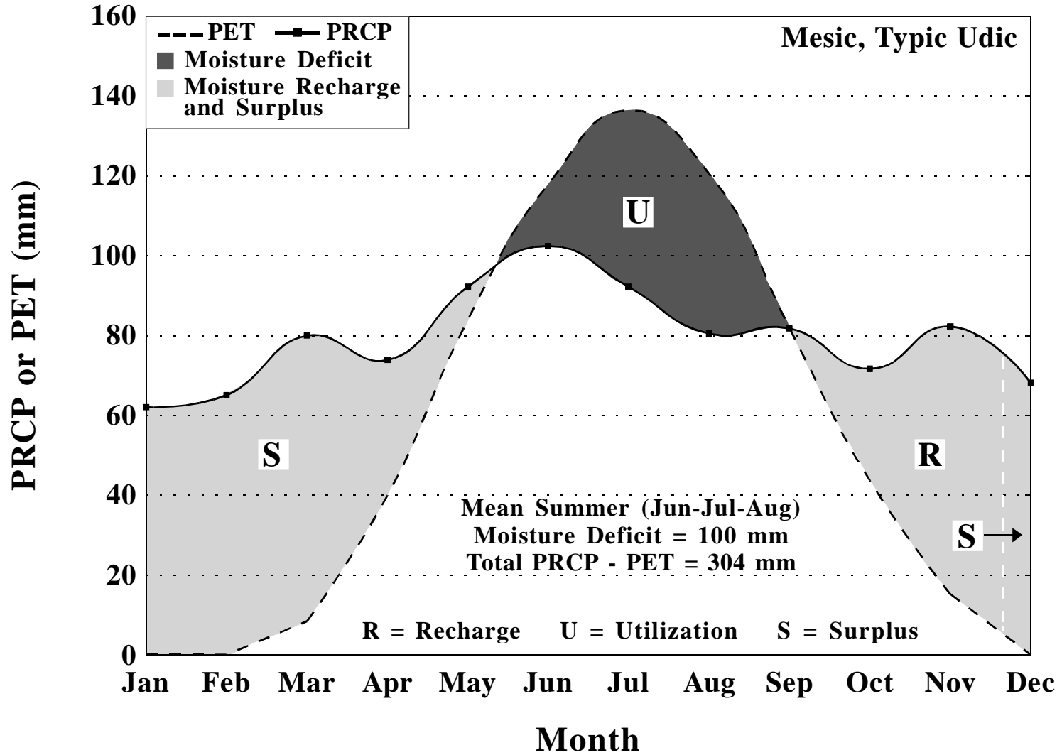
Moisture balance for State College, Pennsylvania, based upon a period of 1961-1990. PET calculated by Newhall Simulation Model (Van Wambeke et al., 1992).
