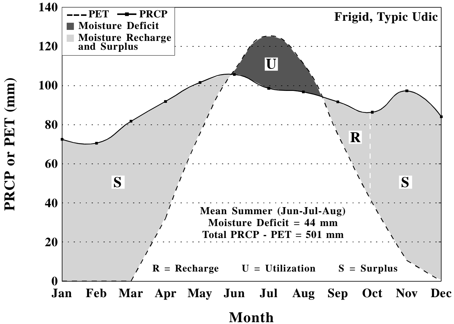
Moisture balance for Montrose, Pennsylvania, based upon a period of 1961-1990. PET calculated by Newhall Simulation Model (Van Wambeke et al., 1992).
