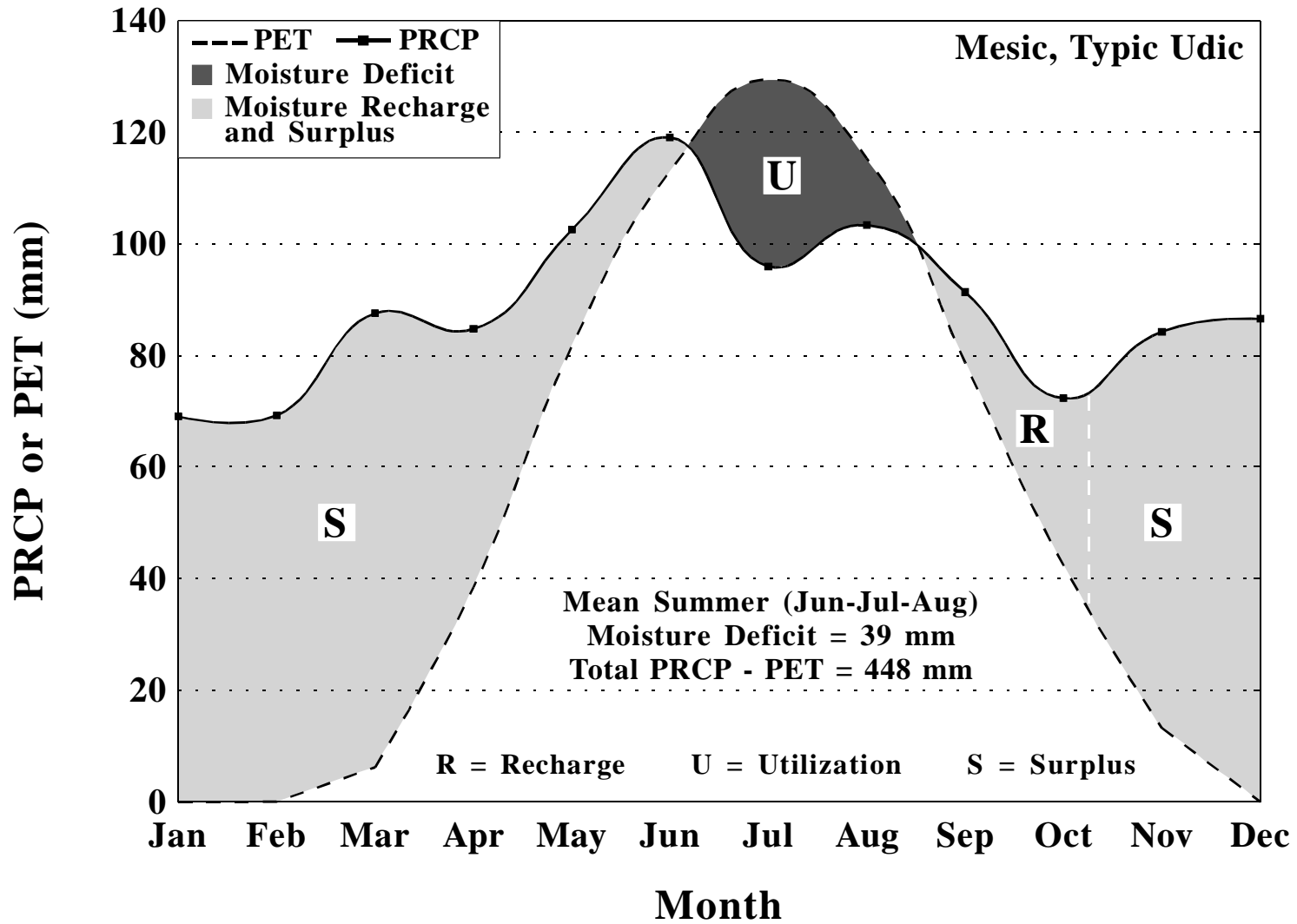
Moisture balance for DuBois FAA Airport, Pennsylvania, based upon a period of 1961-1990. PET calculated by Newhall Simulation Model (Van Wambeke et al., 1992).
