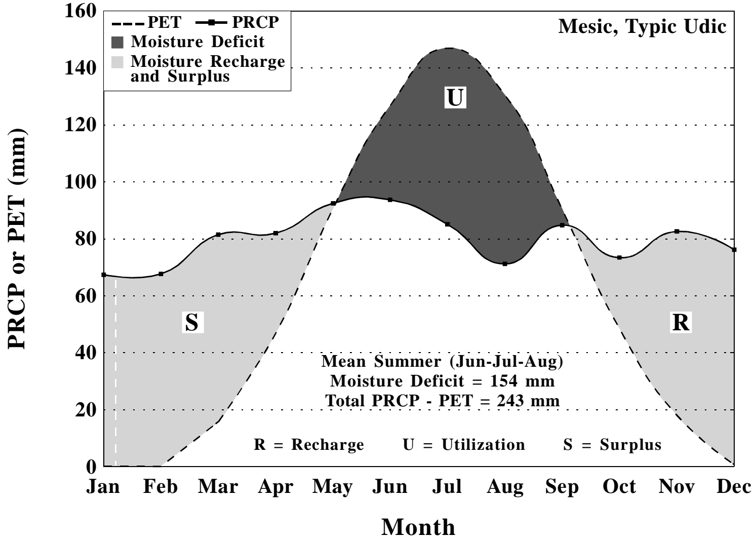
Moisture balance for Shippensburg, Pennsylvania, based upon a period of 1961-1990. PET calculated by Newhall Simulation Model (Van Wambeke et al., 1992).
