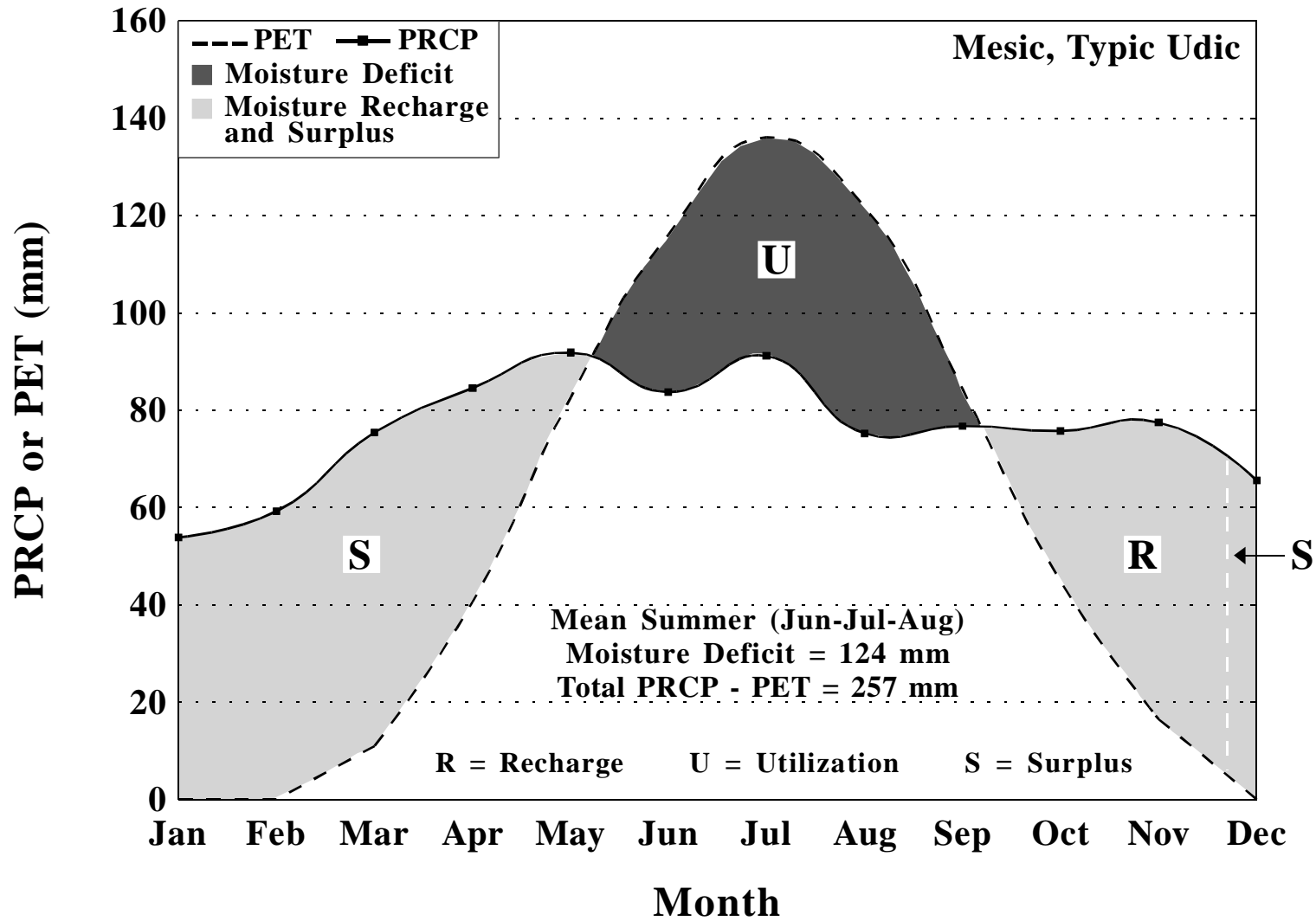
Moisture balance for Everett, Pennsylvania, based upon a period of 1961-1990. PET calculated by Newhall Simulation Model (Van Wambeke et al., 1992).
