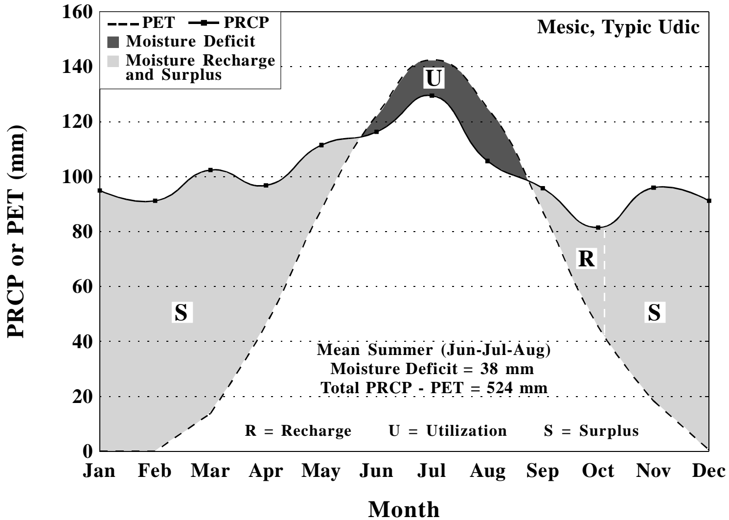
Moisture balance for Johnstown, Pennsylvania, based upon a period of 1961-1990. PET calculated by Newhall Simulation Model (Van Wambeke et al., 1992).
