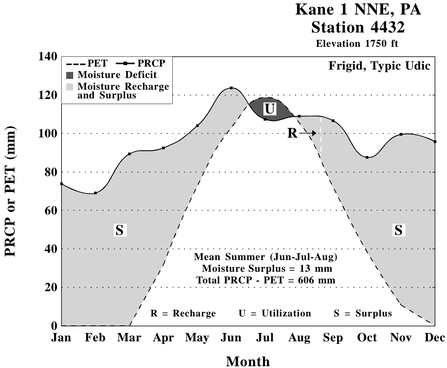
Moisture balance for Kane 1 NNE, Pennsylvania, based upon a period of 1961-1990. PET calculated by Newhall Simulation Model (Van Wambeke et al., 1992).
