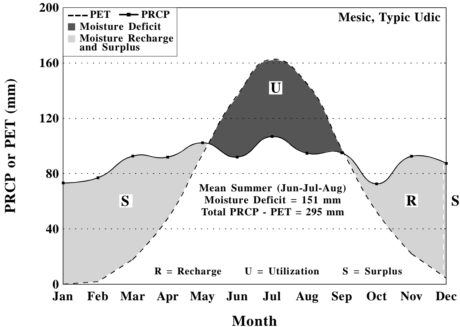
Moisture balance for Marcus Hook, Pennsylvania, based upon a period of 1961-1990. PET calculated by Newhall Simulation Model (Van Wambeke et al., 1992).
