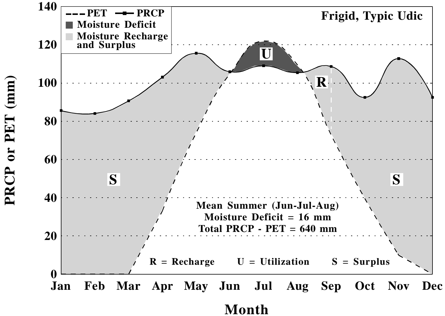
Moisture balance for Tobyhanna, Pennsylvania, based upon a period of 1961-1990. PET calculated by Newhall Simulation Model (Van Wambeke et al., 1992).
