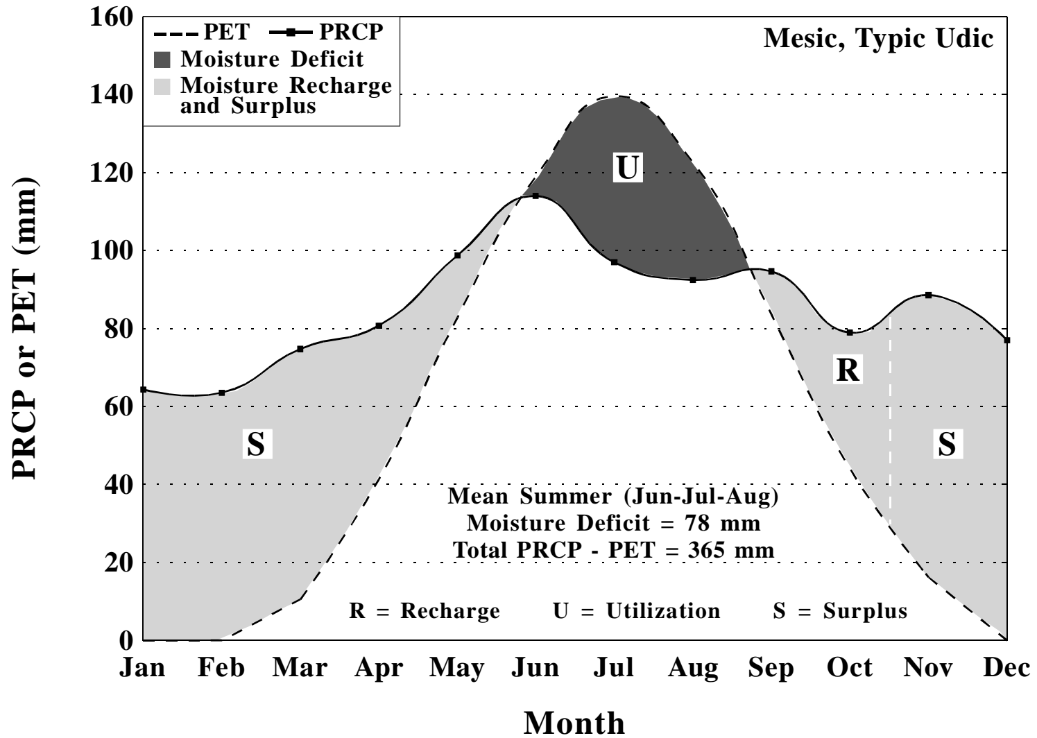
Moisture balance for Selinsgrove 2 S, Pennsylvania, based upon a period of 1961-1990. PET calculated by Newhall Simulation Model (Van Wambeke et al., 1992).
