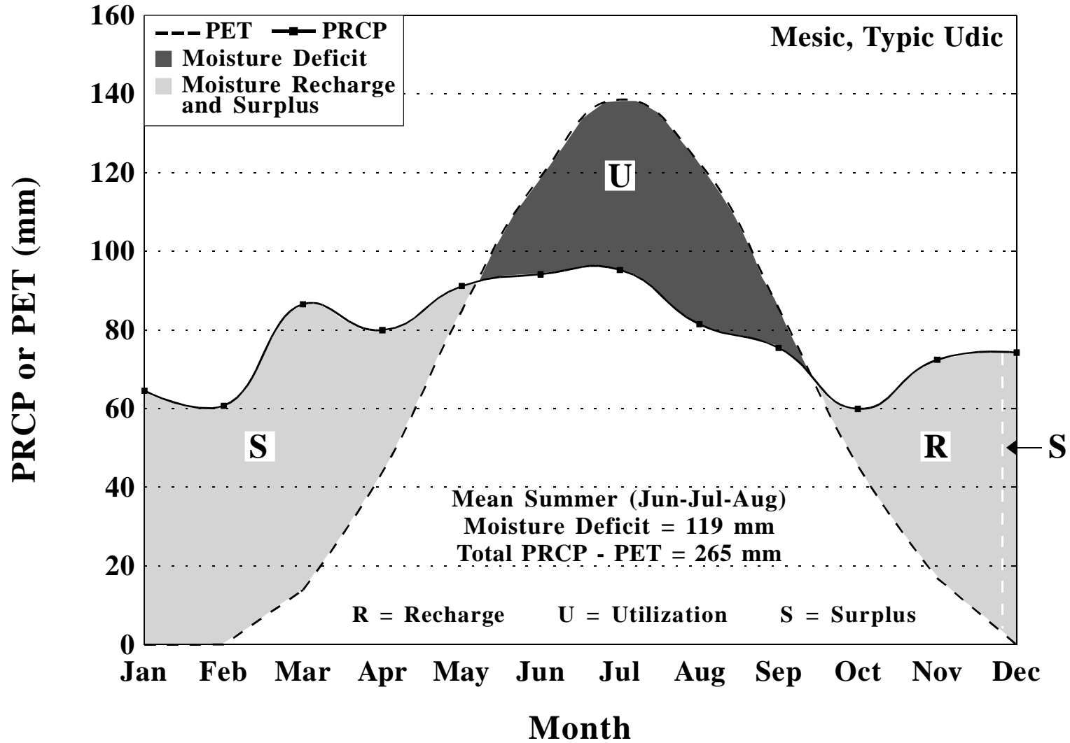
Moisture balance for Pittsburgh WSCMO2 Airport, Pennsylvania, based upon a period of 1961-1990. PET calculated by Newhall Simulation Model (Van Wambeke et al., 1992).
