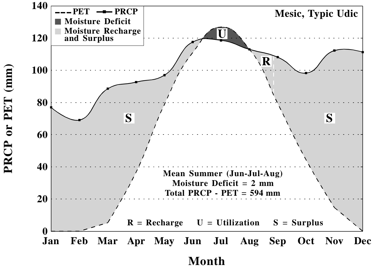
Moisture balance for Corry, Pennsylvania, based upon a period of 1961-1990. PET calculated by Newhall Simulation Model (Van Wambeke et al., 1992).
