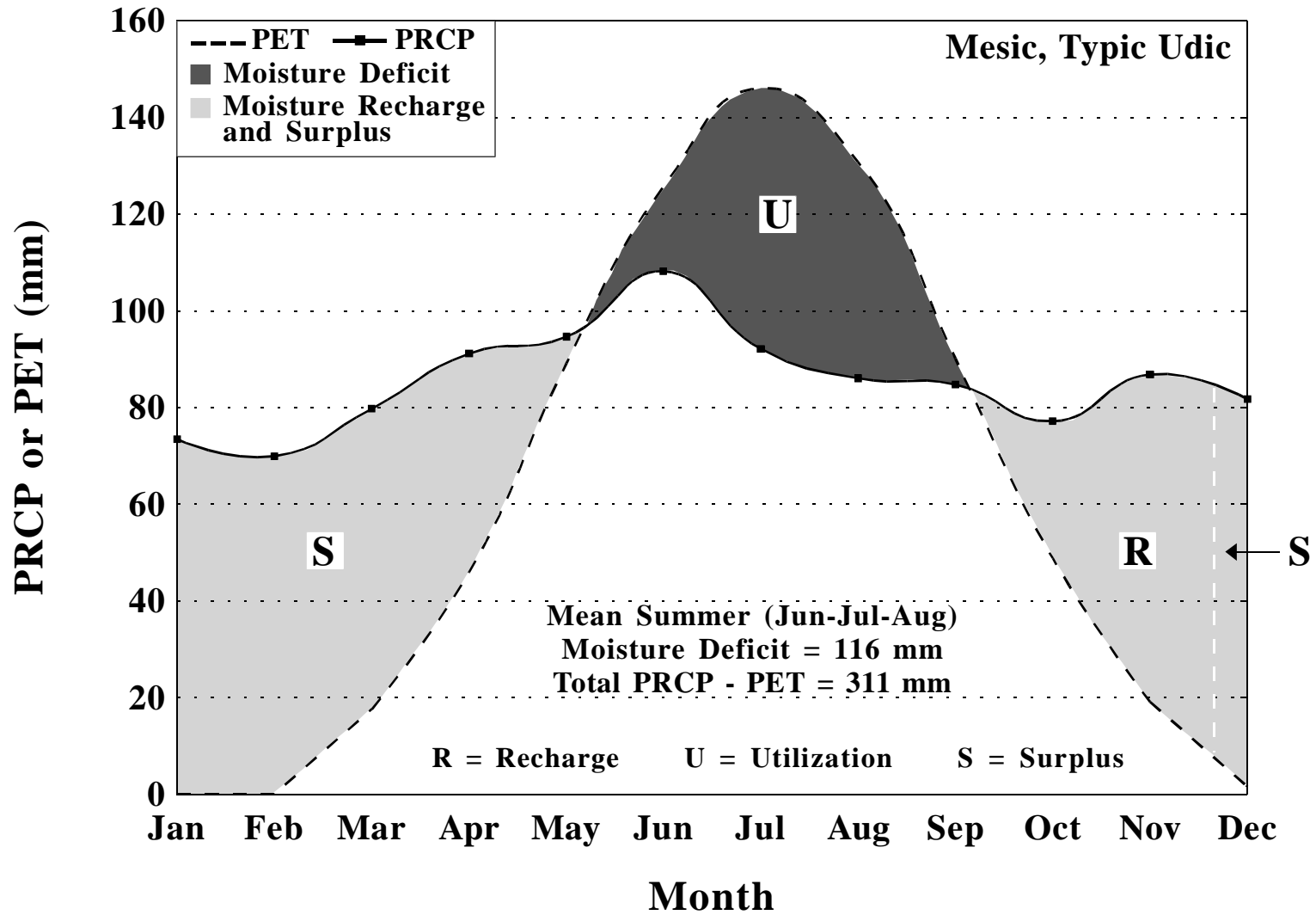
Moisture balance for York 3 SSW Pumping Station, Pennsylvania, based upon a period of 1961-1990. PET calculated by Newhall Simulation Model (Van Wambeke et al., 1992).
