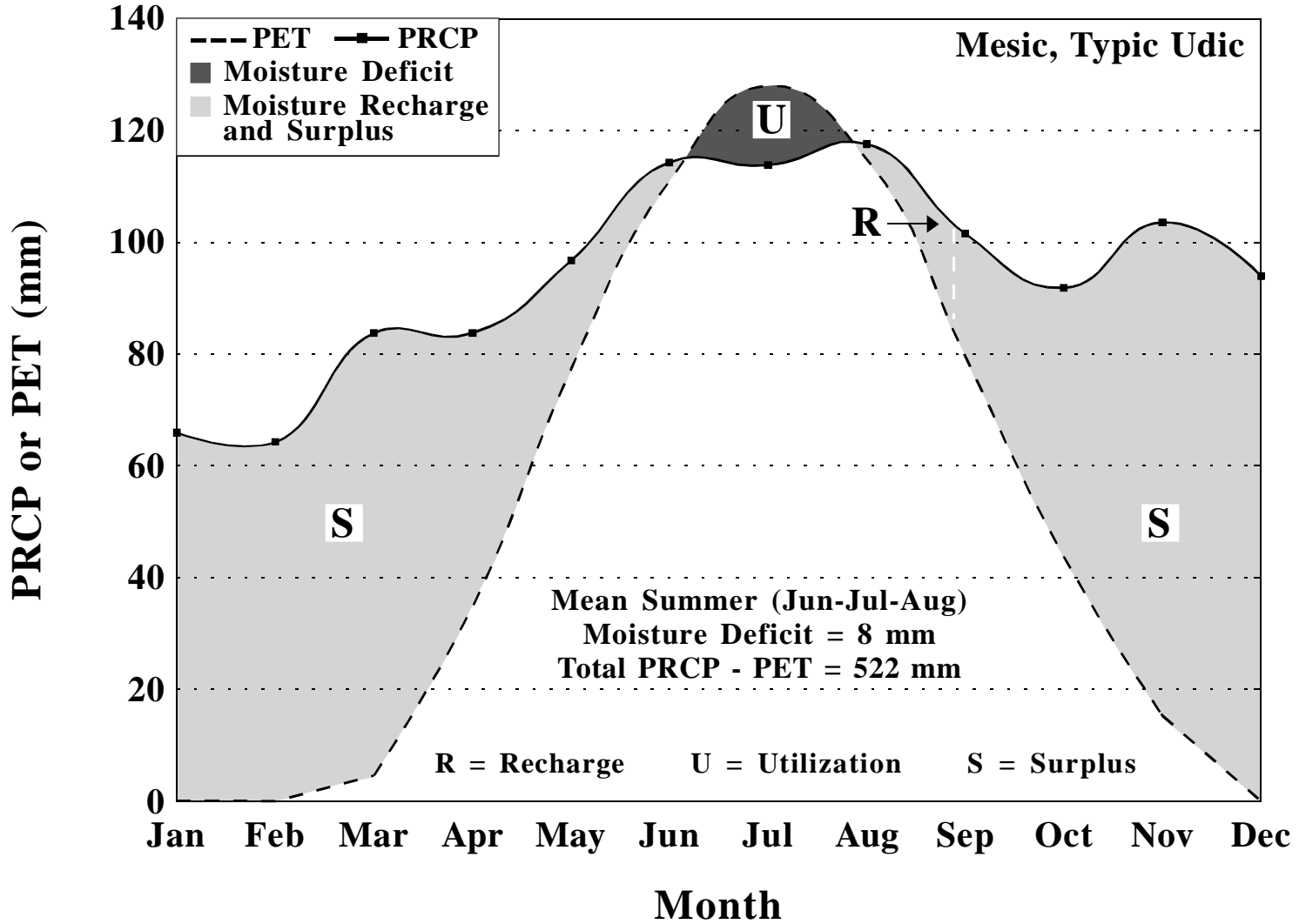
Moisture balance for Meadville 1 S, Pennsylvania, based upon a period of 1961-1990. PET calculated by Newhall Simulation Model (Van Wambeke et al., 1992).
