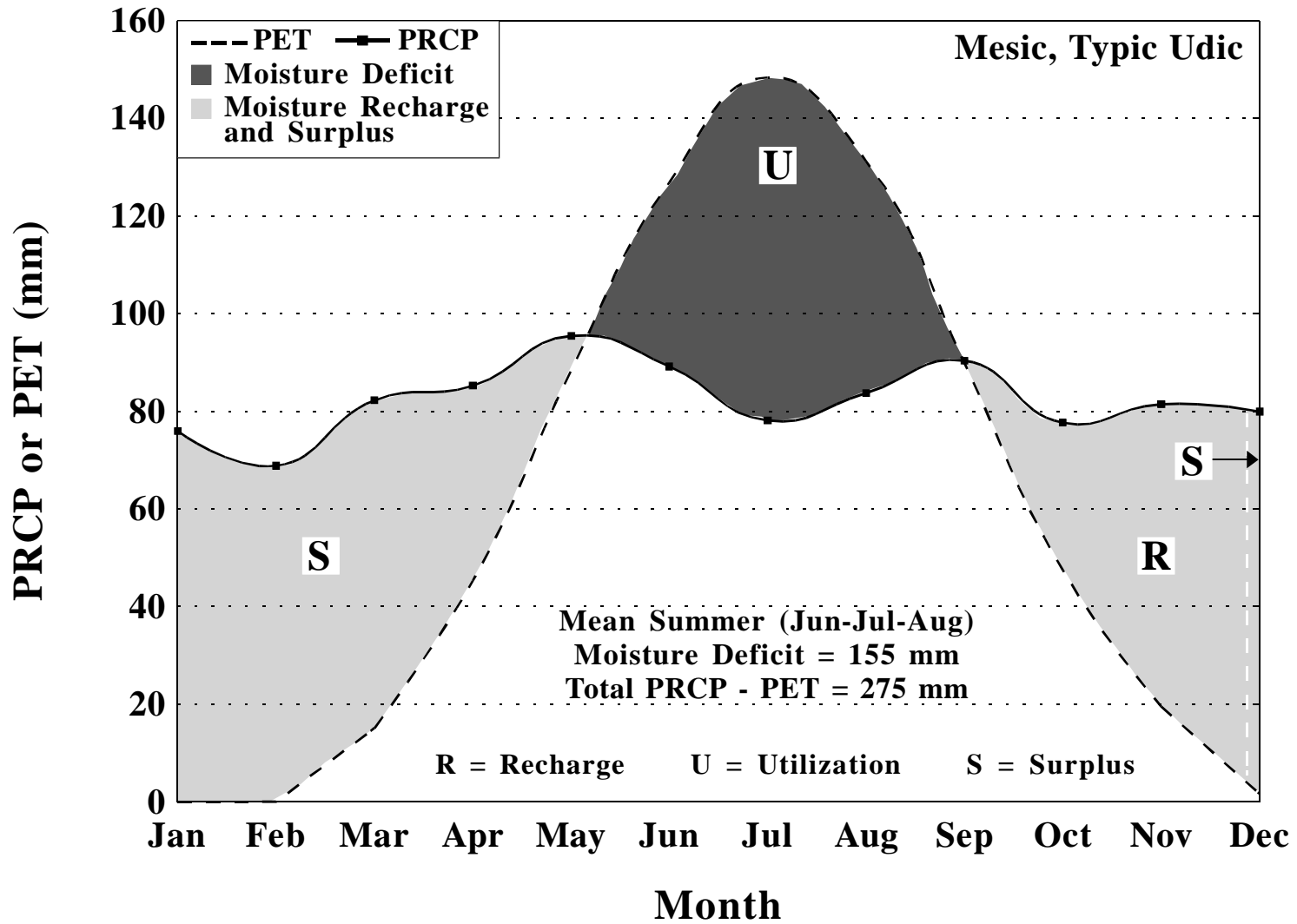
Moisture balance for Hanover, Pennsylvania, based upon a period of 1961-1990. PET calculated by Newhall Simulation Model (Van Wambeke et al., 1992).
