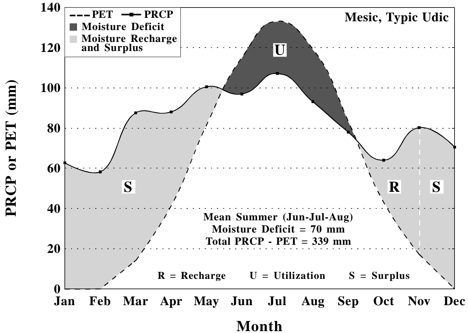
Moisture balance for Waynesburg 1 E, Pennsylvania, based upon a period of 1961-1990. PET calculated by Newhall Simulation Model (Van Wambeke et al., 1992).
