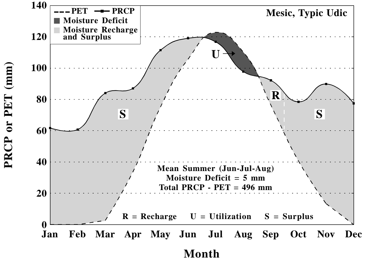
Moisture balance for Ridgway, Pennsylvania, based upon a period of 1961-1990. PET calculated by Newhall Simulation Model (Van Wambeke et al., 1992).
