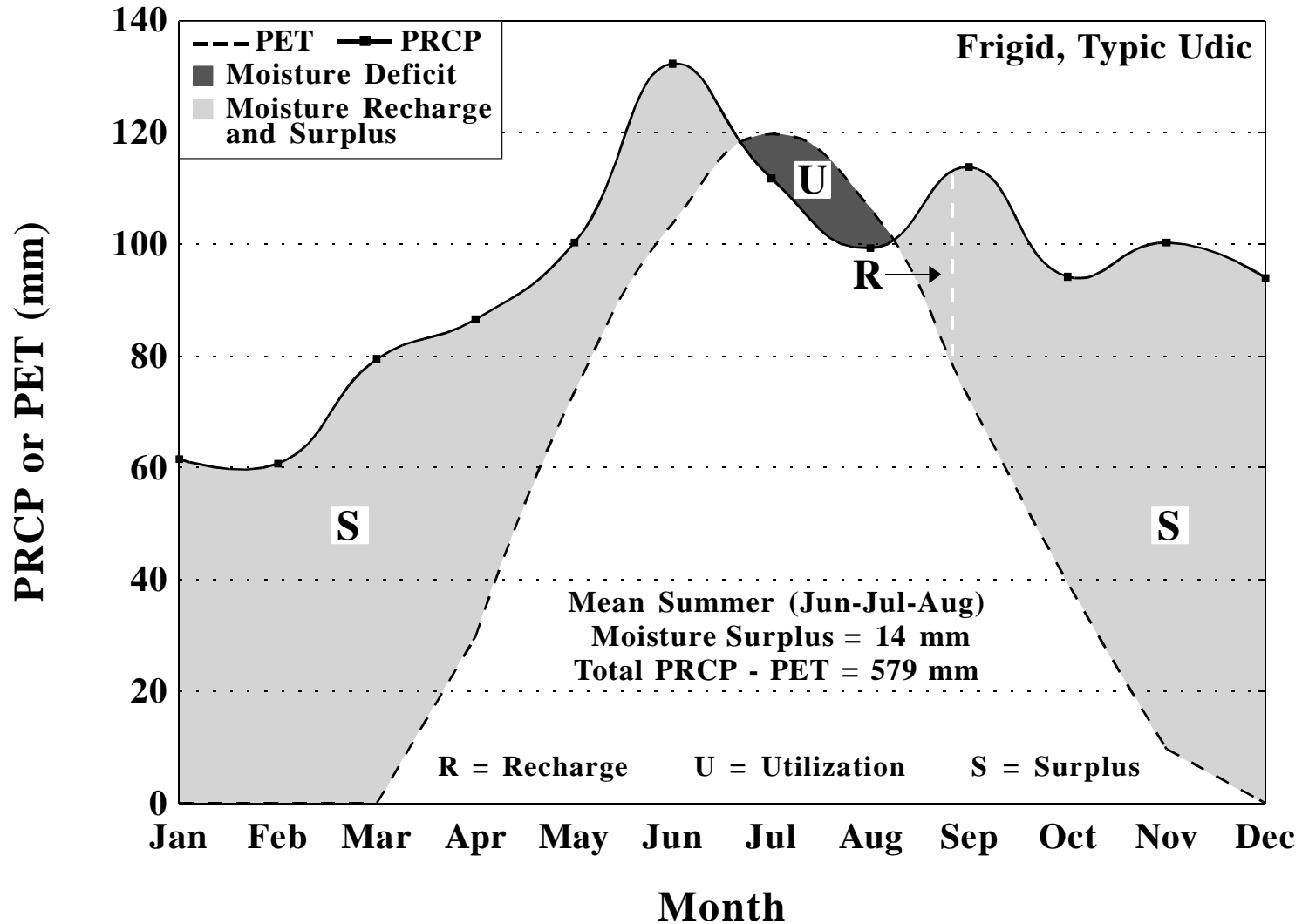
Moisture balance for Bradford 4 W RES 1, Pennsylvania, based upon a period of 1961-1990. PET calculated by Newhall Simulation Model (Van Wambeke et al., 1992).
