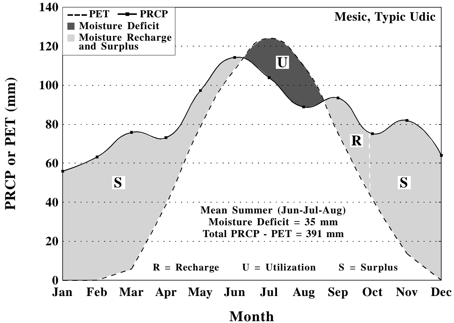
Moisture balance for Philipsburg 8 E, Pennsylvania, based upon a period of 1961-1990. PET calculated by Newhall Simulation Model (Van Wambeke et al., 1992).
