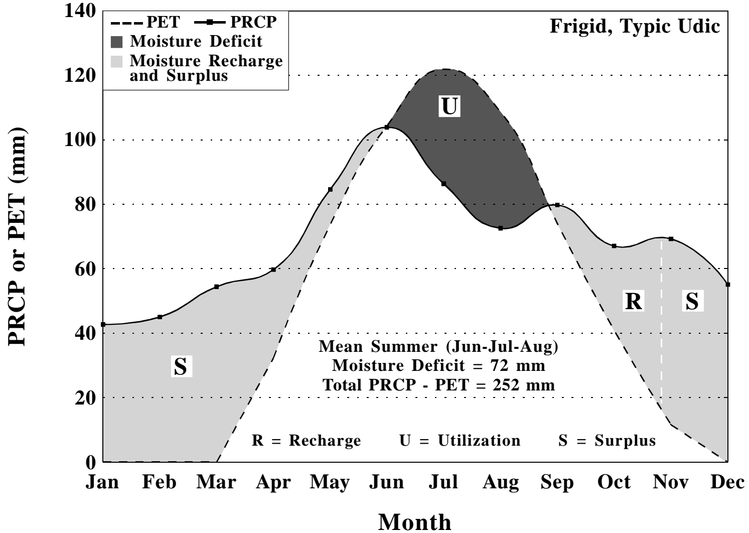
Moisture balance for Wellsboro 3 S, Pennsylvania, based upon a period of 1961-1990. PET calculated by Newhall Simulation Model (Van Wambeke et al., 1992).
