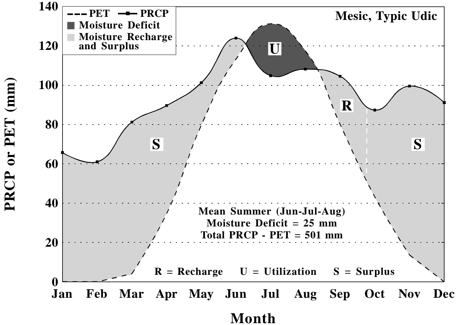
Moisture balance for Warren 1 SSW, Pennsylvania, based upon a period of 1961-1990. PET calculated by Newhall Simulation Model (Van Wambeke et al., 1992).
